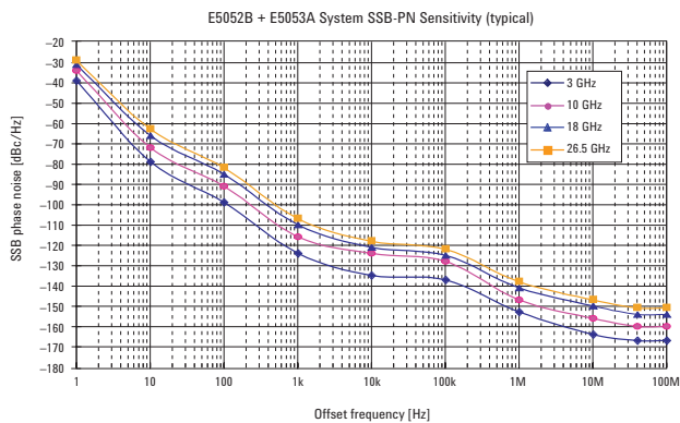
Figure 10-2. System phase noise sensitivity (E5053A + E5052B) (typical)
