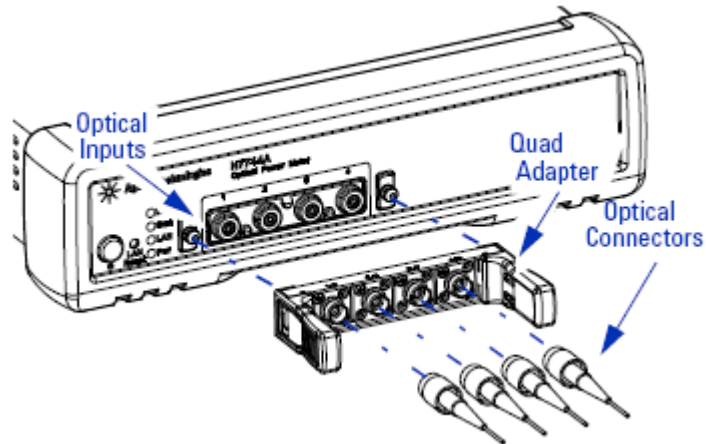
Figure 21 Connecting Optical Fibers
