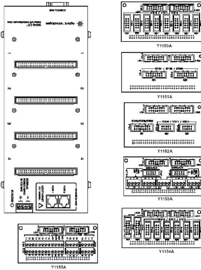
Figure 1. The Y1150A – Y1155A Distribution Boards
