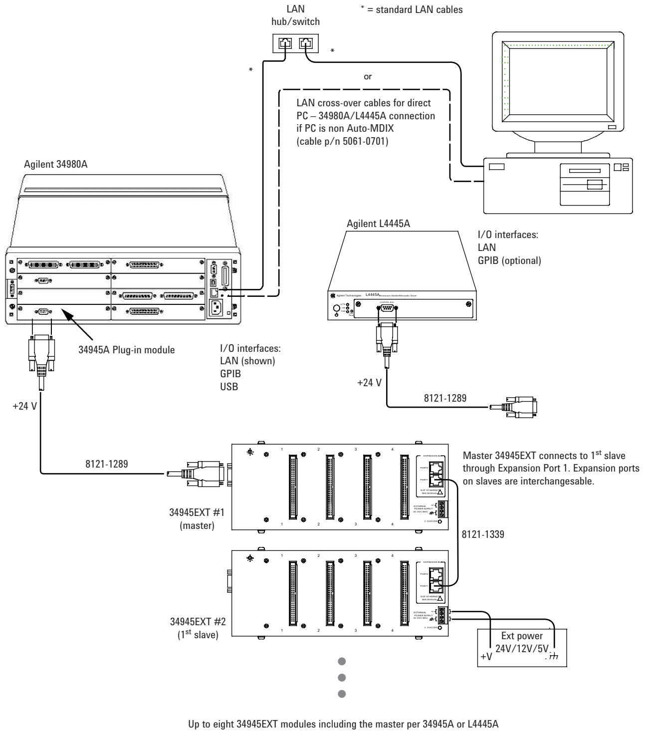
Figure 2. 34945A and L4445A External Connections
