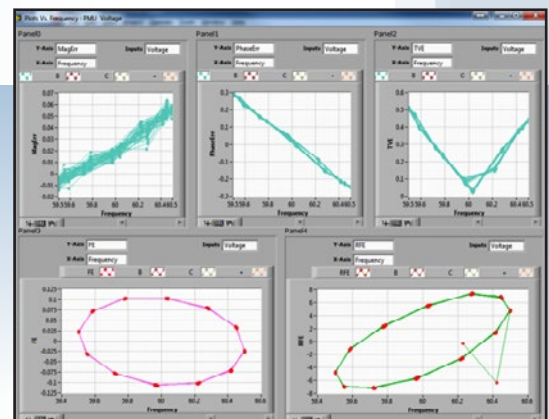
Plots of tested PMU measurement errors versus frequency
